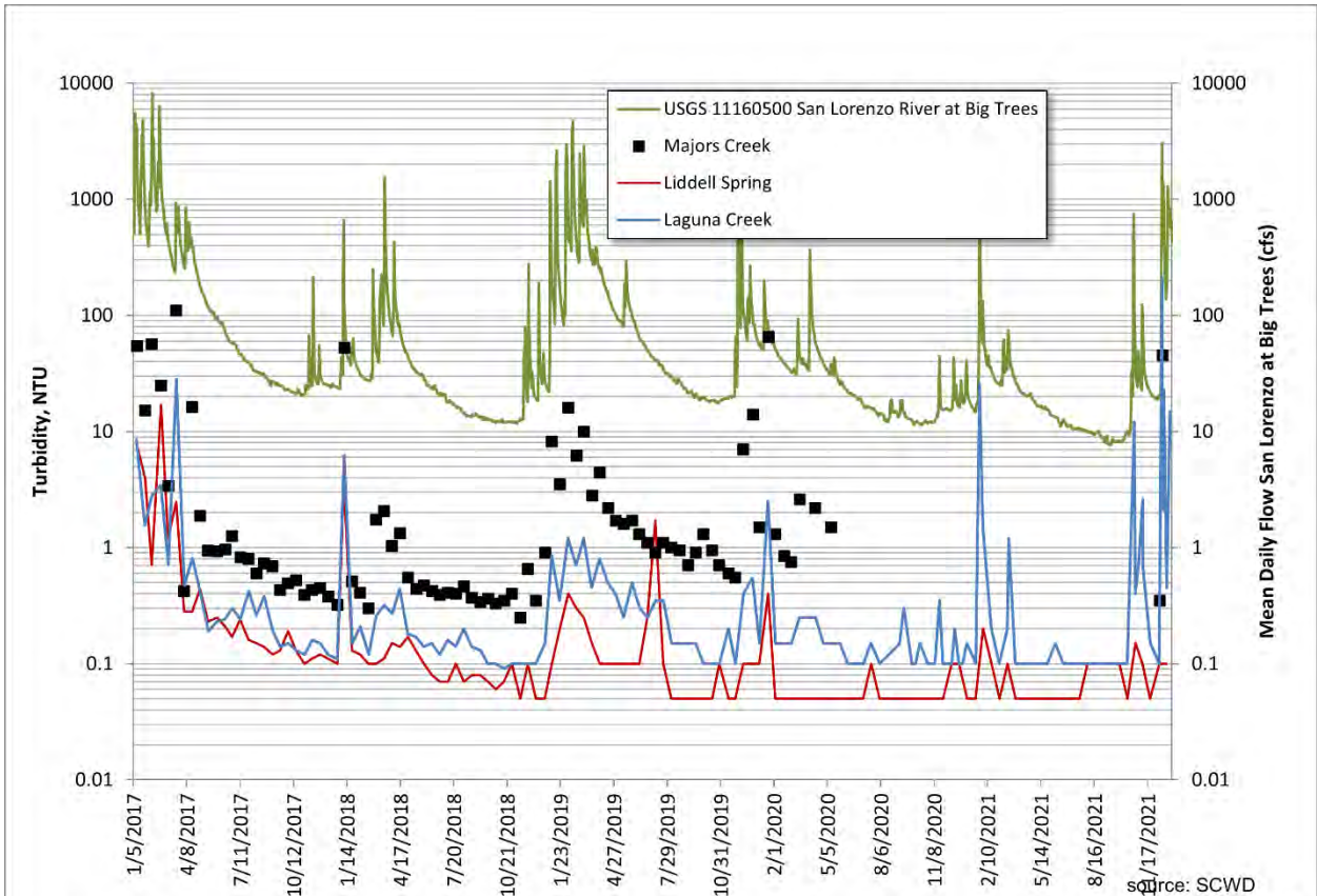
Figure 5-5 Turbidity in SCWD's North Coast Sources, 2017-2021 Turbidity data is collected at varying intervals. Mean daily flows from San Lorenzo River at Big Trees are shown for reference to sediment transport conditions. Majors Creek was off line from May 2020 - November 2021.
