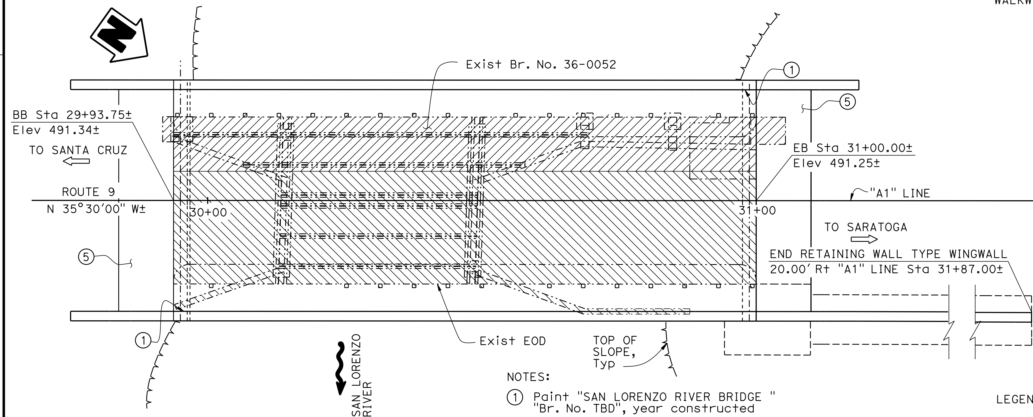
PLAN 1" = 10'
