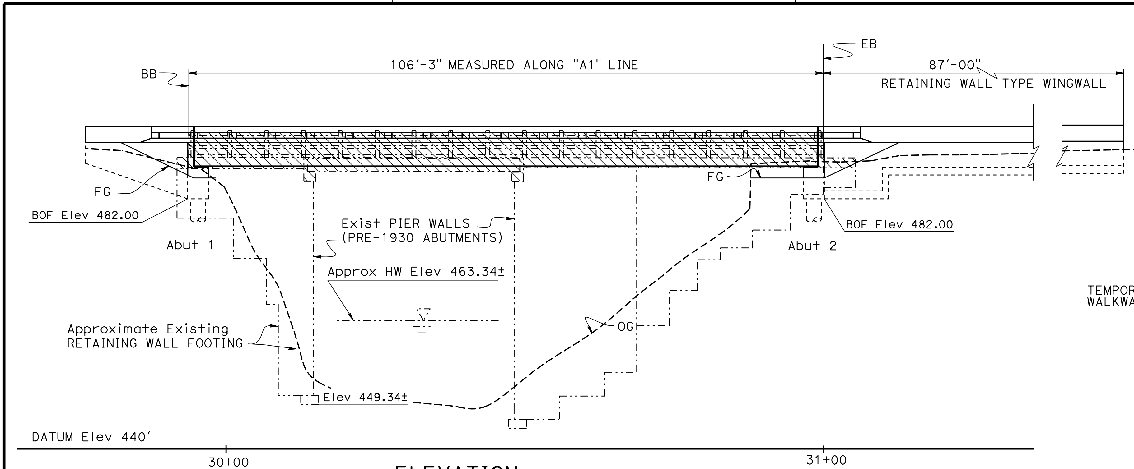
ELEVATION 1" = 10'
