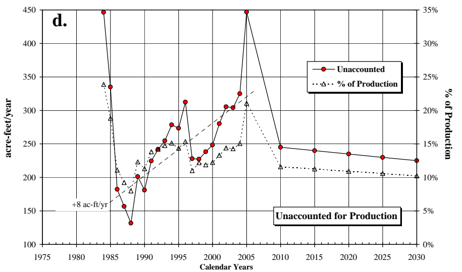
Figure 2-3 SLVWD Historical and Projected Water Use Trends, 1977-2030
