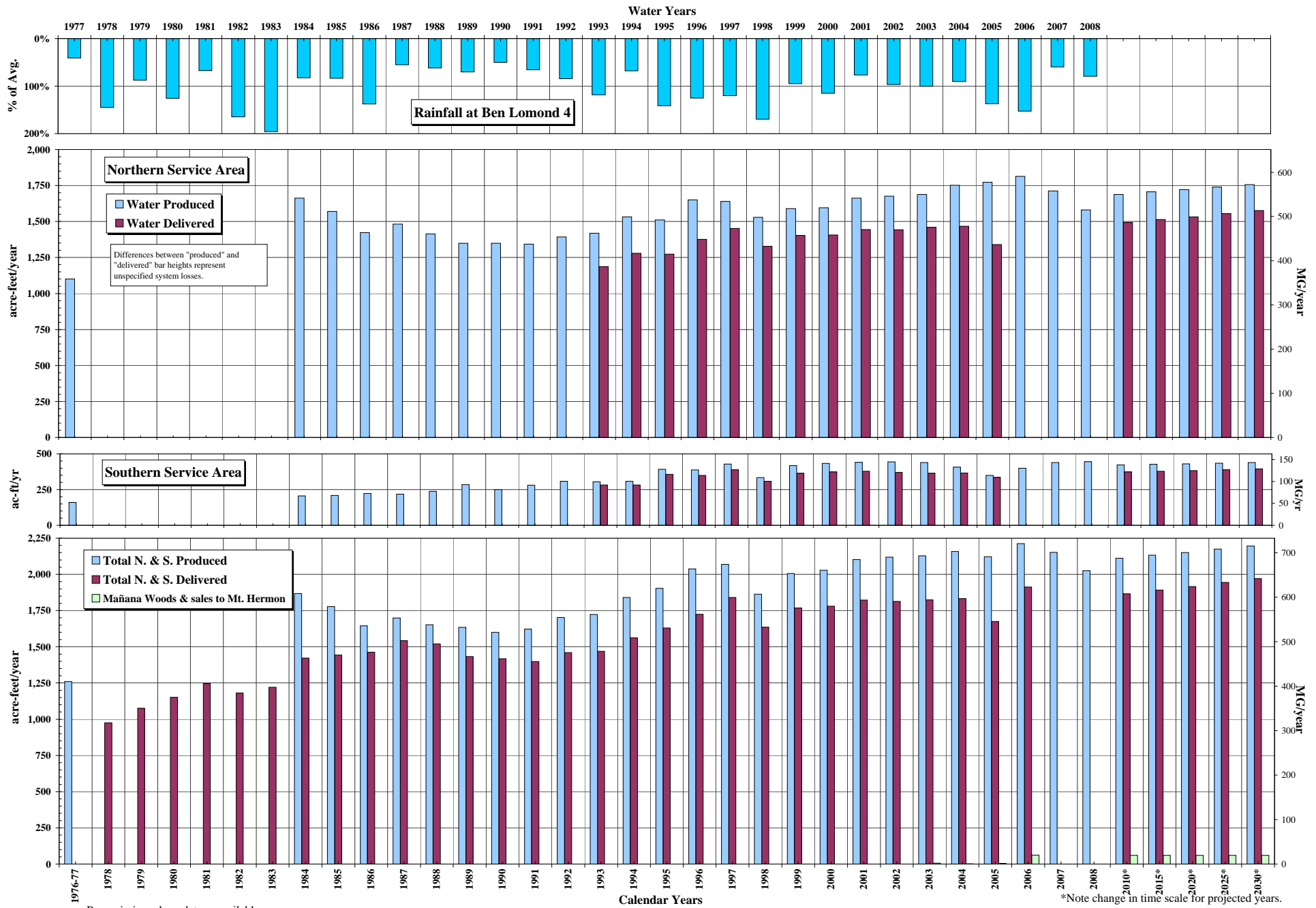
Figure 2-1 SLVWD Historical and Projected Water Production and Deliveries, 1977-2030
